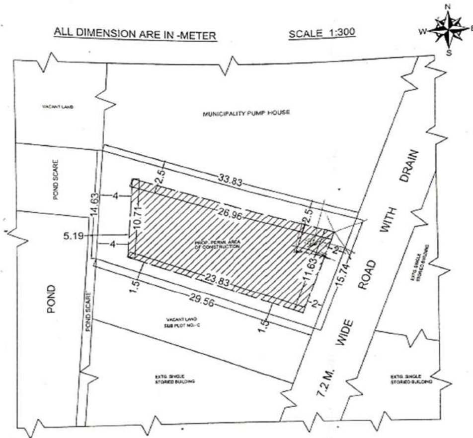
SITE PLAN
